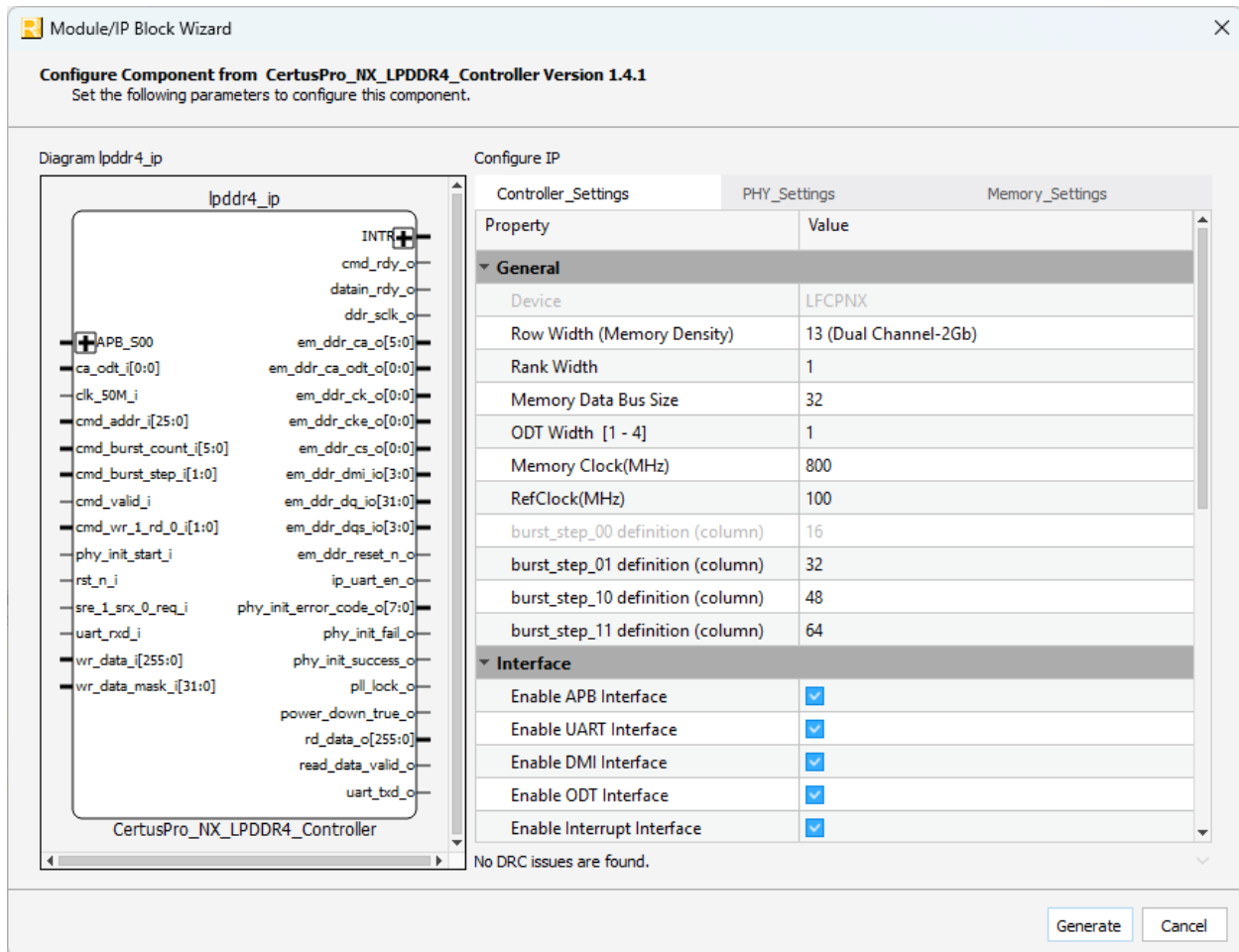
Figure 6.1 GUI Controller Settings
