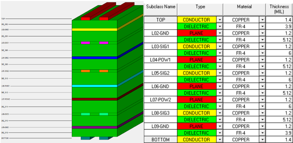
Figure 9.4 Reference PCB Stack information
